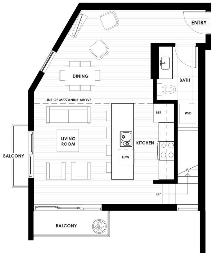
FOURTH FLOOR
